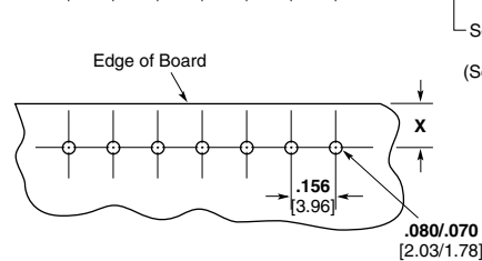
Recommended Mounting Hole Pattern for .062 [1.57] Thk. PC Board
